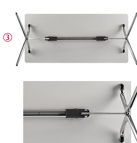
Detail of mechanism of Enclose and Blocked, patented by ACTIU
